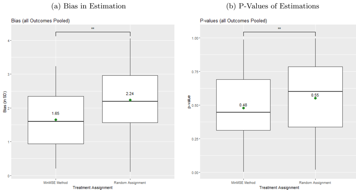
Figure 3: Comparison of Precision: (Absolute) Bias and P-Values of Estimations
