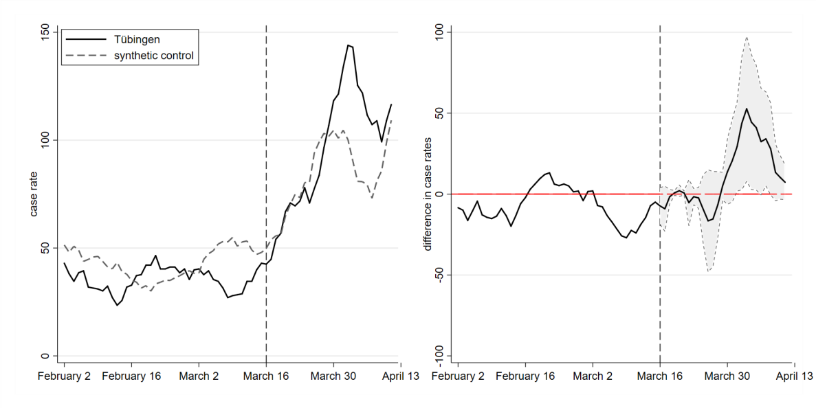
Figure 1: Seven-day case rates for donor pool Baden-Württemberg
