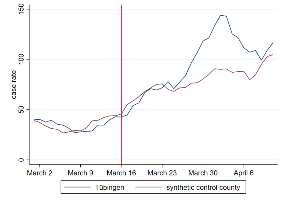
Figure 8: Seven-day case rates for predictor set 2 and 'leave all out'
